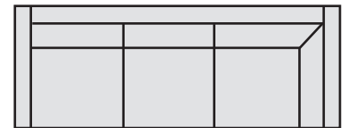
76532 Left Arm Corner Sofa Total W 92" D 35" H 35" Seat D 22" H 18" W 75" Arm Height 26"
