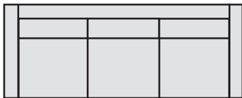
76530 Sofa Total W 88" D 35" H 35" Seat D 22" H 18" W 79" Arm Height 26"
