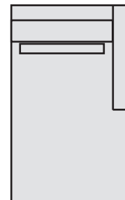
62561 Right Arm Chaise Total W 44" D 71" H 34" Seat D 51" H 15" W 44" Arm Height 24"
