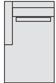
62562 Left Arm Chaise Total W 44" D 71" H 34" Seat D 51" H 15" W 44" Arm Height 24"
