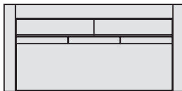
62530 Sofa Total W 90" D 44" H 34" Seat D 24" H 15" W 81" Arm Height 24"
