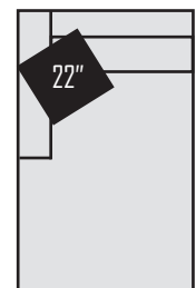
49562 Left Arm Chaise Total W 40" D 65" H 37" Seat D 50" H 19" W 32" Arm Height 26"
