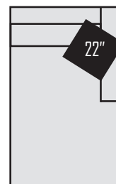
49561 Right Arm Chaise Total W 40" D 65" H 37" Seat D 50" H 19" W 32" Arm Height 26"
