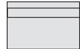
49538 Armless 2 Seater Sofa Total W 60" D 40" H 37" Seat D 24" H 19" W 60"
