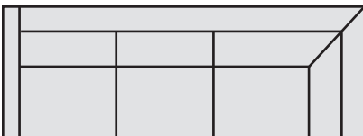
46532 Left Arm Corner Sofa Total W 107" D 37" H 36" Seat D 22" H 18" W 85" Arm Height 27"
