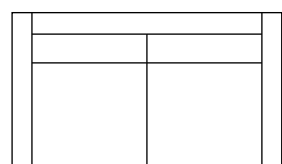
46535 APARTMENT SOFA TOTAL W70" D37" H36" SEAT W63" D22" H18" ARMS --- --- H27"
