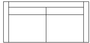
46530 JUDE SOFA TOTAL W85" D37" H36" SEAT W78" D22" H18" ARMS --- --- H27"
